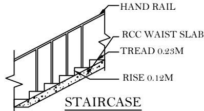
STAIRCASE
