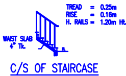
C/S OF STAIRCASE
