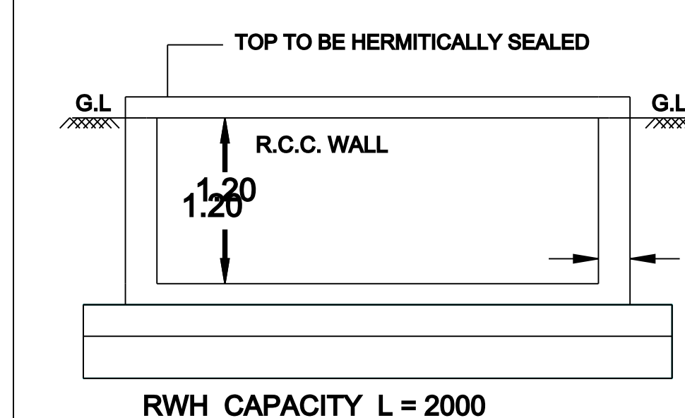
RWH SECTION
