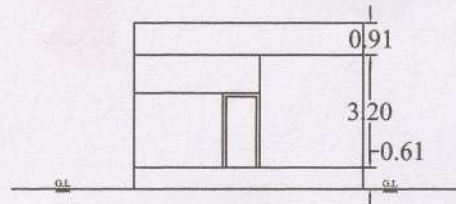
FRONT ELEVATION
