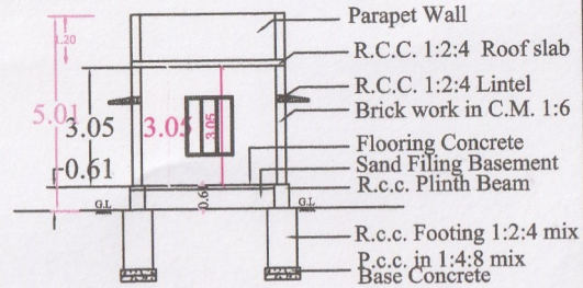
SECTION - "AB"
