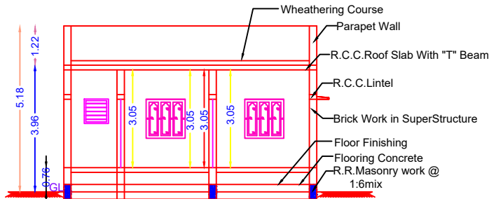
SECTION ON "PQ" SCALE 1:100
