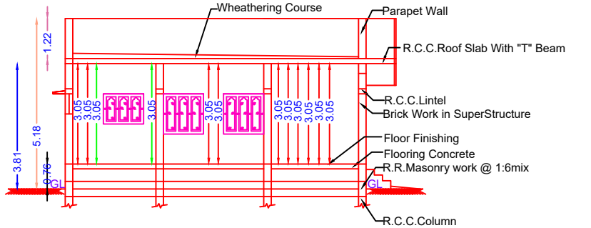
SECTION ON "PQ"
