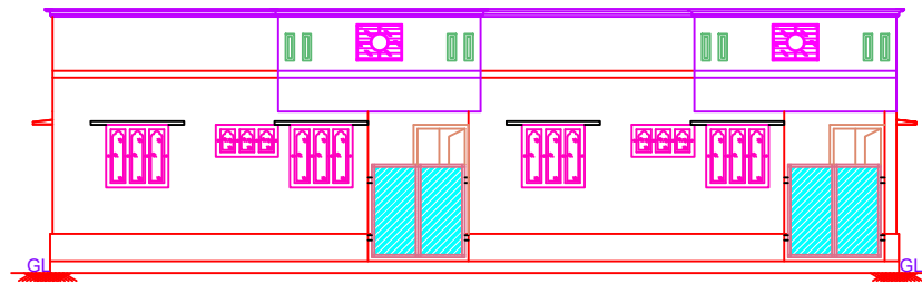
FRONT ELEVATION
