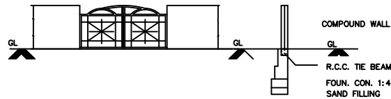
SECTION ON "XX"
