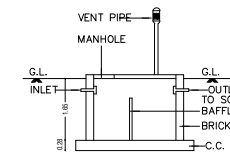
SECTION OF SEPTIC TANK
