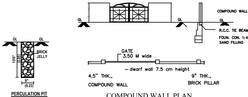
COMPOUND WALL PLAN
