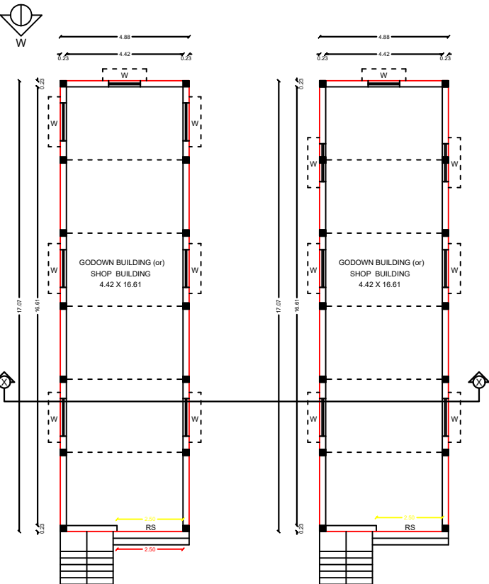
PROPOSED UNDER GROUND FLOOR PLAN
