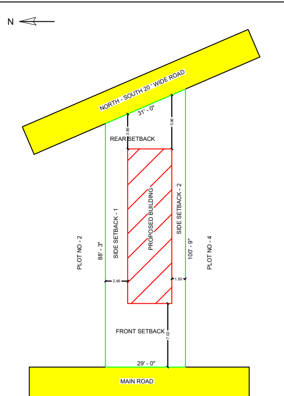
SITE PLAN
