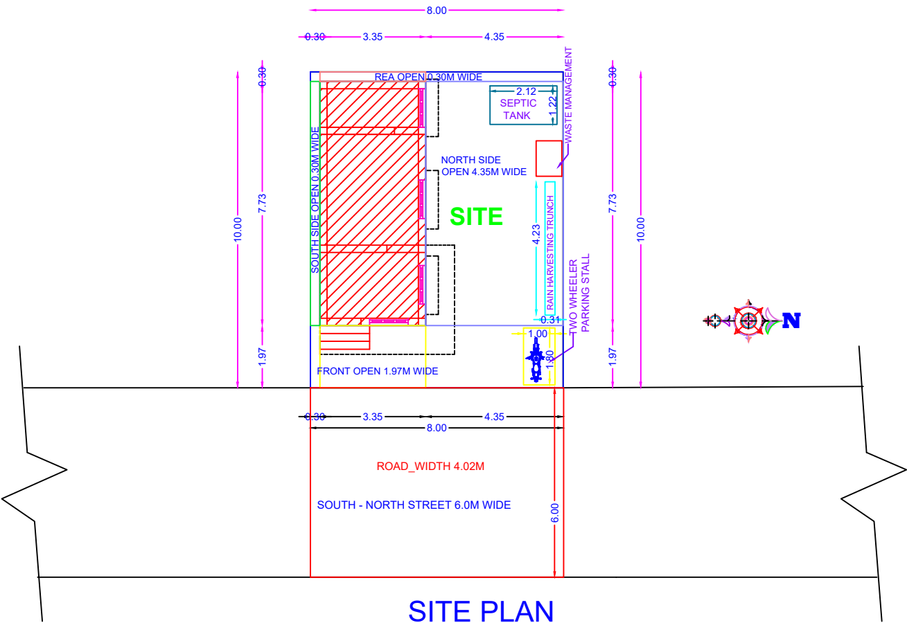
SITE PLAN
