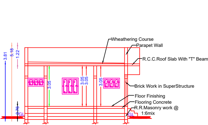
SECTION ON "PQ"
