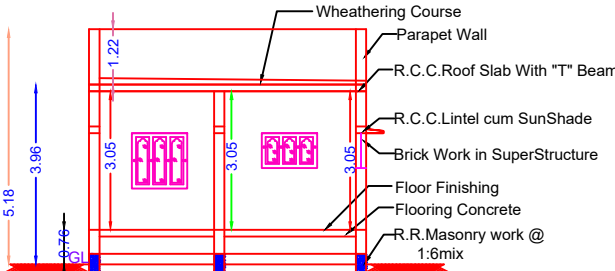
SECTION ON "PQ" SCALE 1:100
