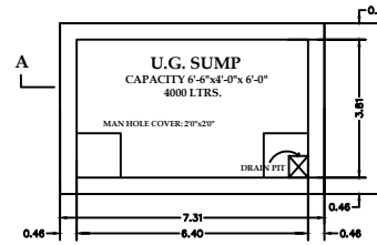
SUMP DETAIL SCALE 1"=4'0"
