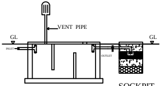
SEPTICTANK DETAILS
