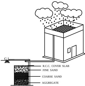
RAIN WATER HARVESTING ARRANGEMENT SAVE RAIN WATER AVOID WATER SCARCITY FOR FUTURE
