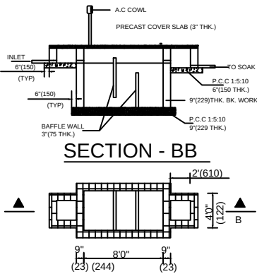
PLAN OF SEPTIC TANK
