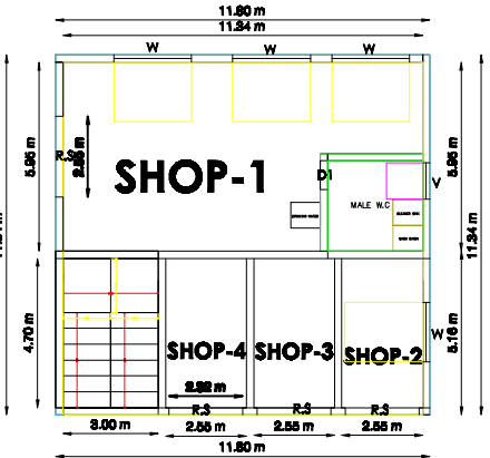
GROUN FLOOR PLAN
