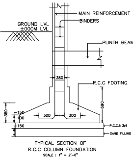
TYPICAL SECTION OF R.C.C. COLUMN FOUNDATION
