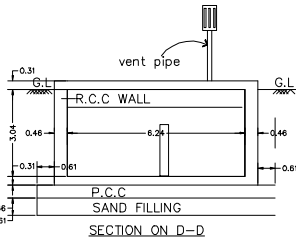
SECTION ON D-D
