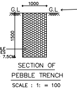
SECTION OF PEBBLE TRENCH
