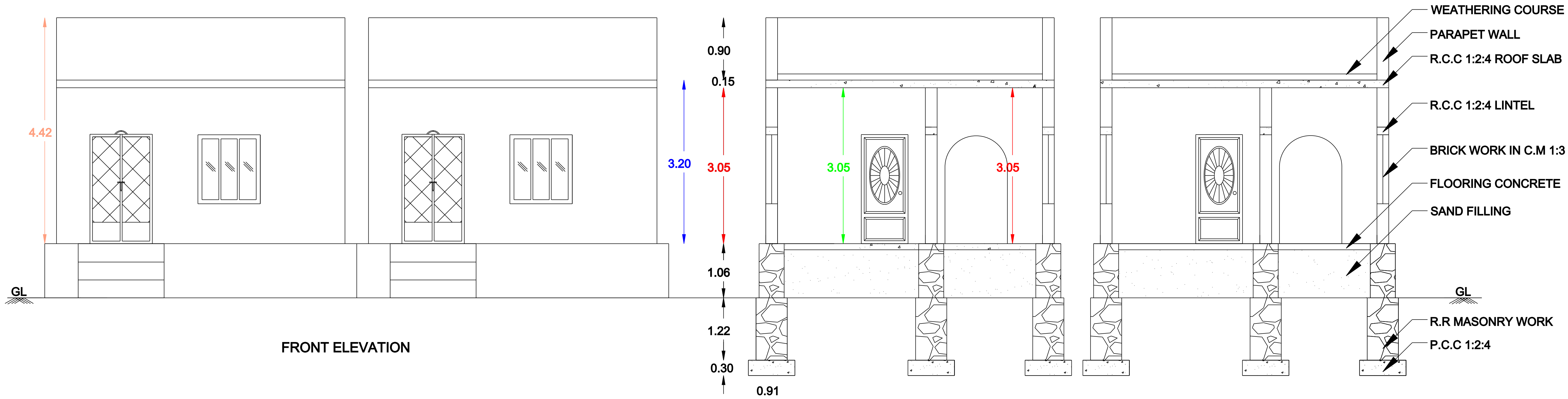
SECTION ON AA
