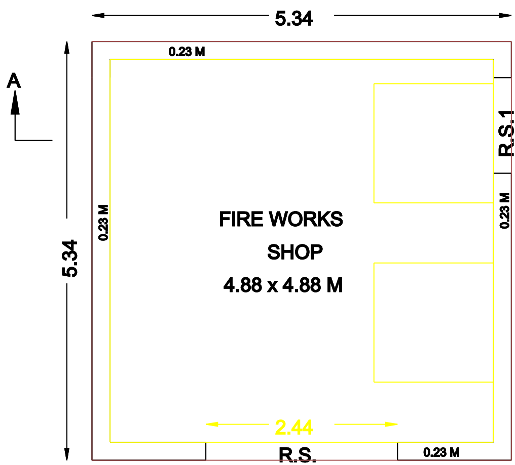
PROPOSED FIRE WORKS SHOP
