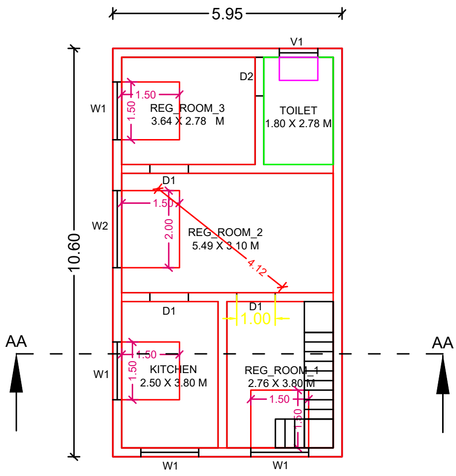
PLAN - FIRST FLOOR (NEW PROPOSAL)
