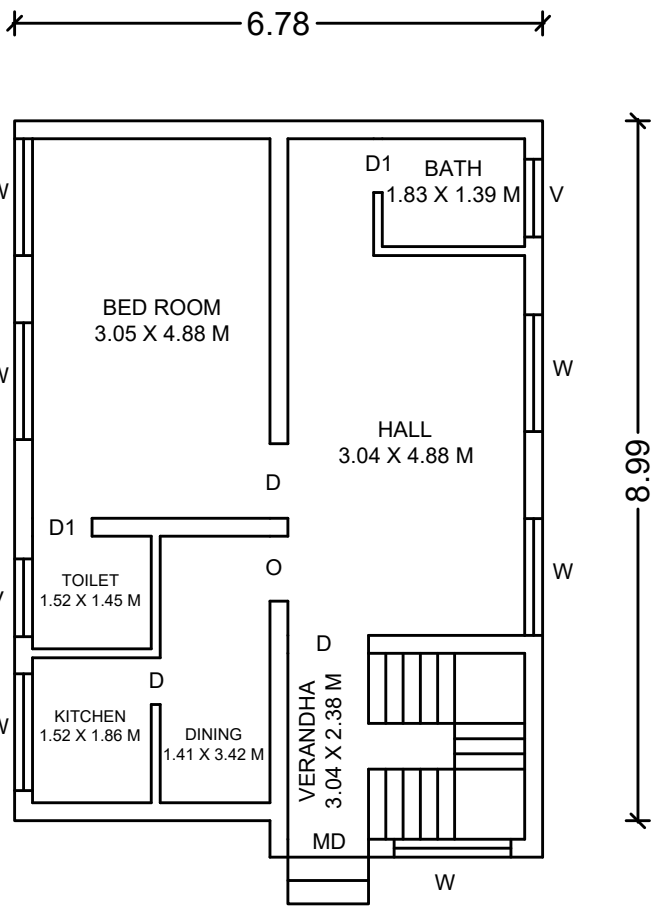
OLD APPROVED GROUND FLOOR PLAN(Date:1.10.2015)
