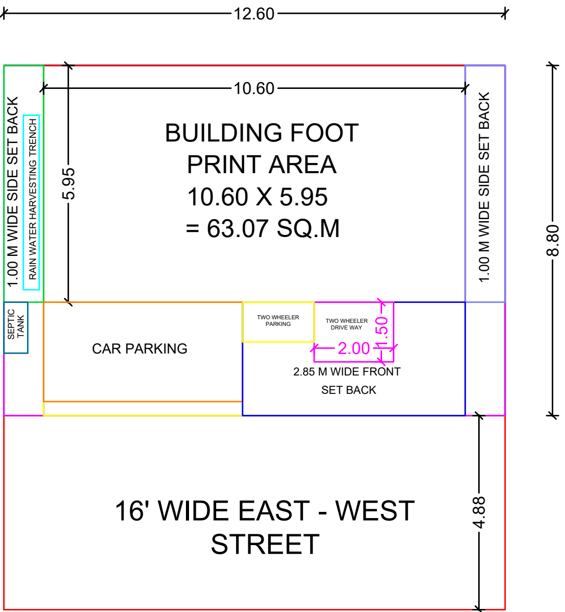
SITE PLAN DETAILS SCALE :- 1:100
