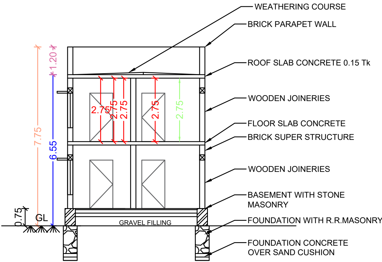
SECTION VIEW"AA"
