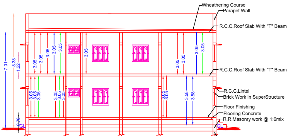
SECTION ON "PQ" SCALE 1:100
