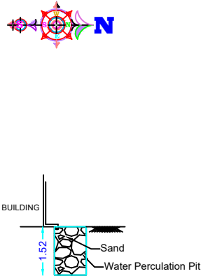
DETAILS OF RAIN WATER PERCOLATION PIT (SCALE 1:100)
