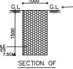
SECTION OF PEBBLE TRENCH
