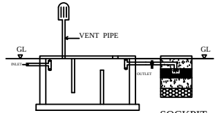
SEPTICTANK DETAILS
