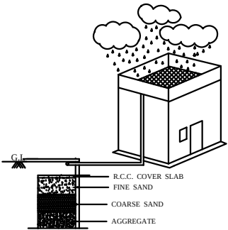
RAIN WATER HARVESTING ARRANGEMENT SAVE RAIN WATER AVOID WATER SCRCITY FOR FUTURE
