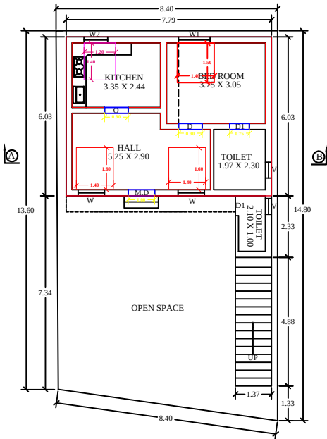
GROUND FLOOR PLAN SCALE :- 1 : 1
