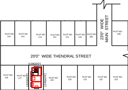
LOCATION PLAN 1:400
