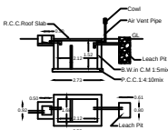
DETAILS OF SEPTIC TANK
