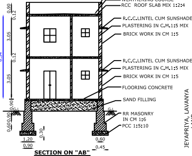
SECTION ON "AB"
