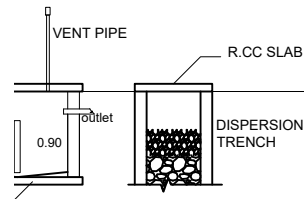
SEPTIC TANK SECTION
