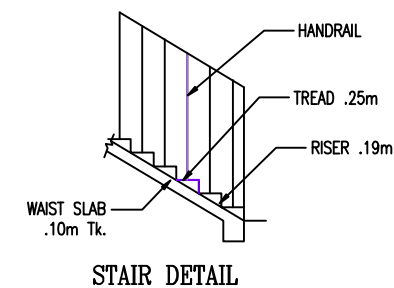
STAIR DETAIL
