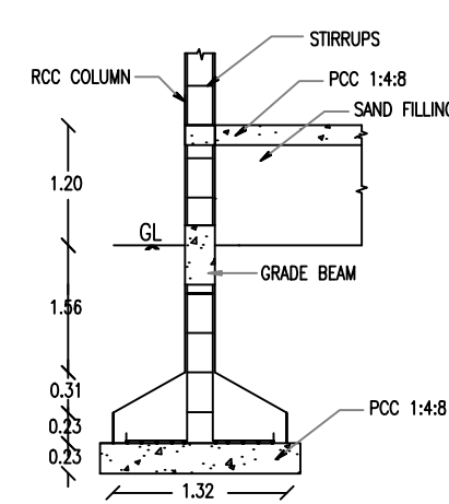
COLUMN DETAILS
