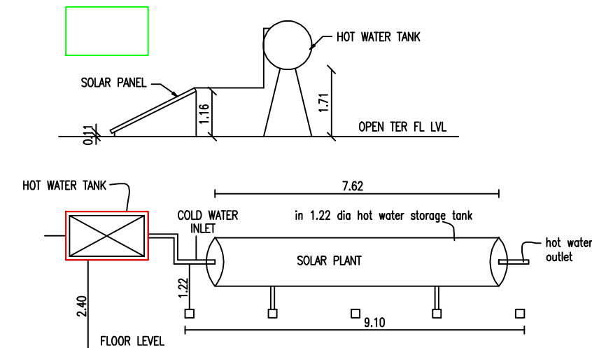
SOLAR WATER HEATER PLANT DETAILS
