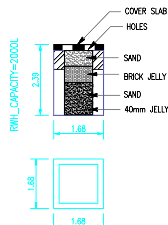
RAIN WATER COLLECTION TANK
