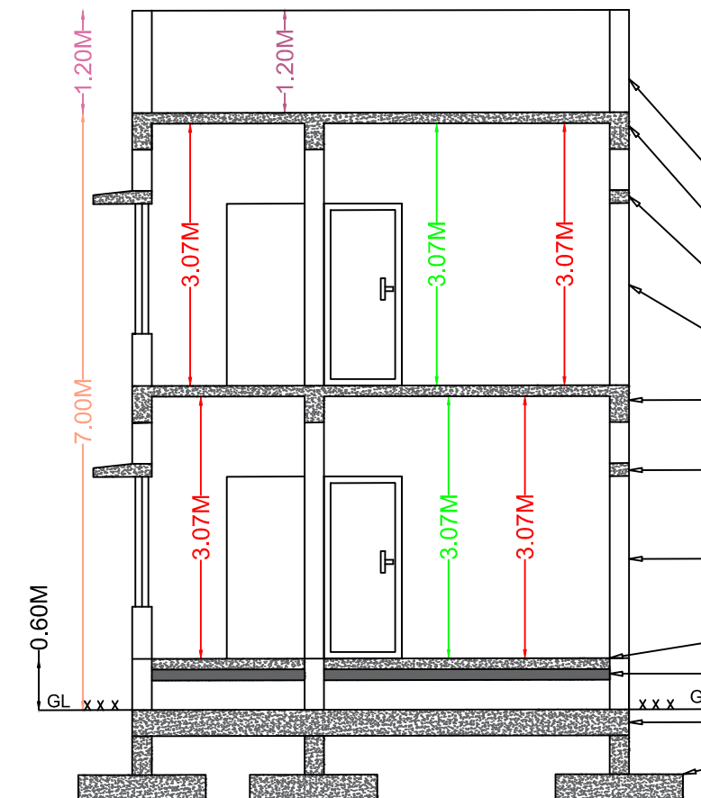
SECTION AB
