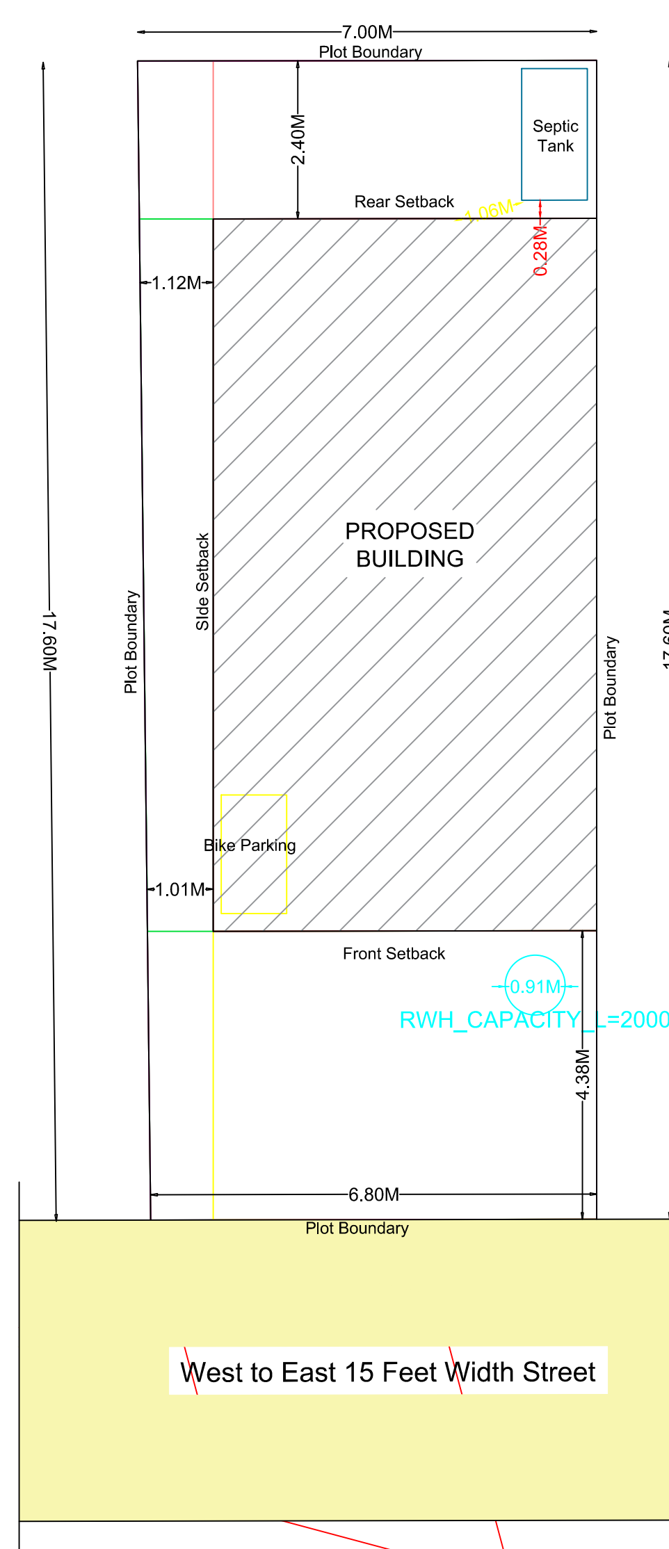
SITE PLAN
