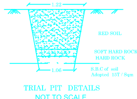
TRIAL PIT DETAILS NOT TO SCALE
