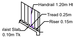
AILS OF STAIR CASE (SCALE 1:100)
