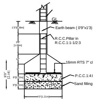
FOUNDATION DETAILS
