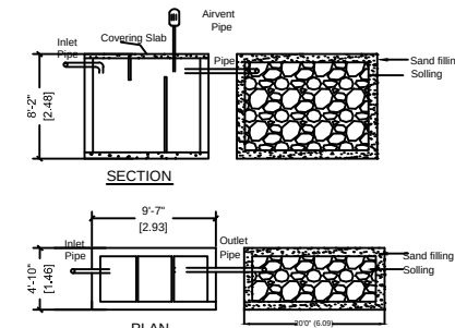
DETAILS OF SEPTIC TANK & DISPERSION TRENCH
