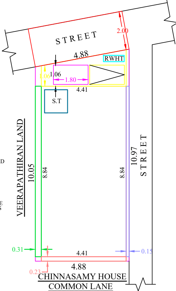
SITE PLAN
