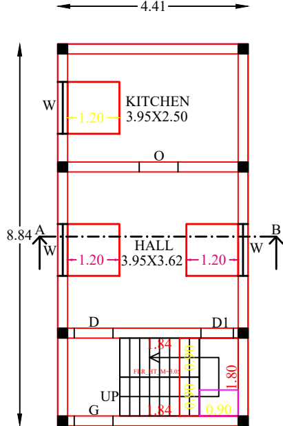
PLAN
