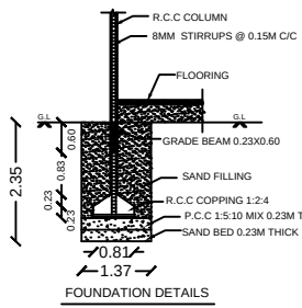
FOUNDATION DETAILS
