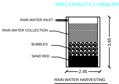
RWH_CAPACITY_L=2000LTRS
