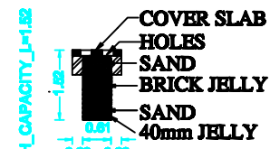
SECTION OF RAIN WATER COLLECTION TANK
