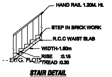
STAIR DETAIL
