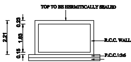
SECTION ON "U.G.SUMP"
