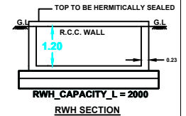
RW SECTION
