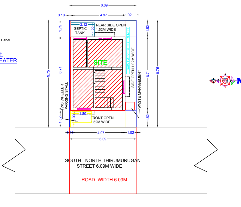
SITE PLAN
