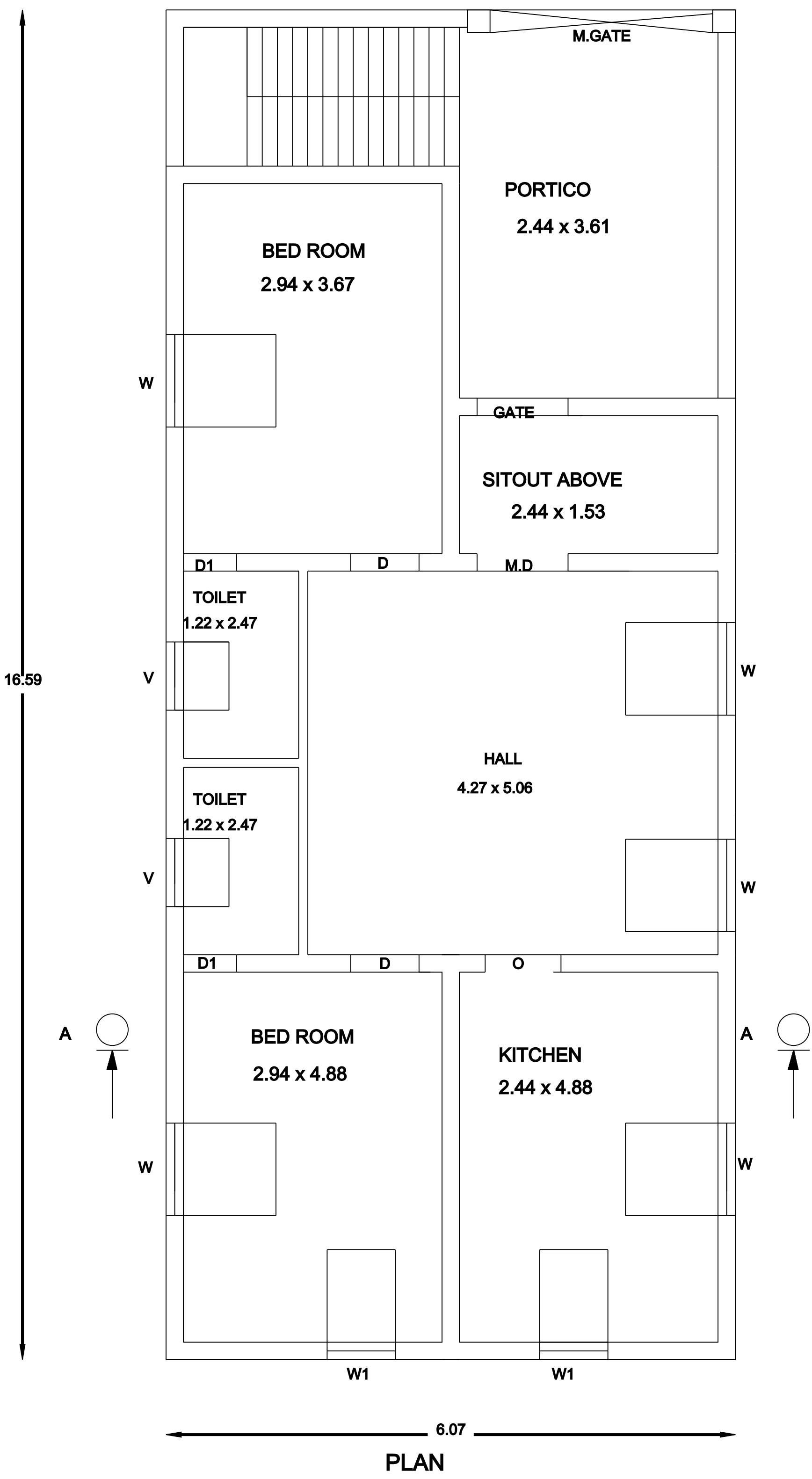
PLAN
