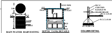
RAIN WATER HARVESTING
