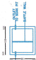
PLAN SEPTIC TANK
