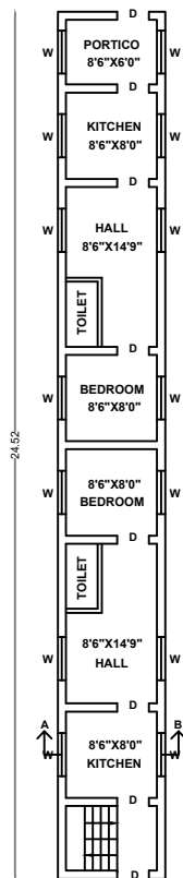
GROUND FLOOR PLAN
