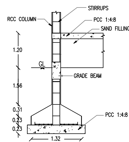
COLUMN DETAILS
