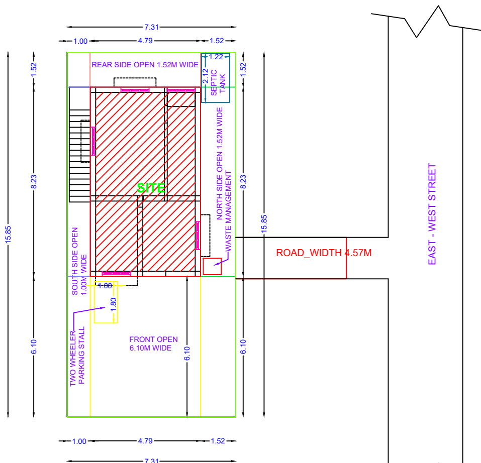
SITE PLAN
