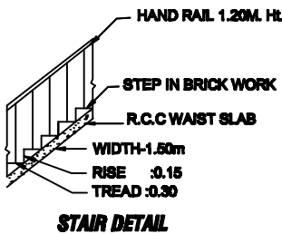
STAIR DETAIL
