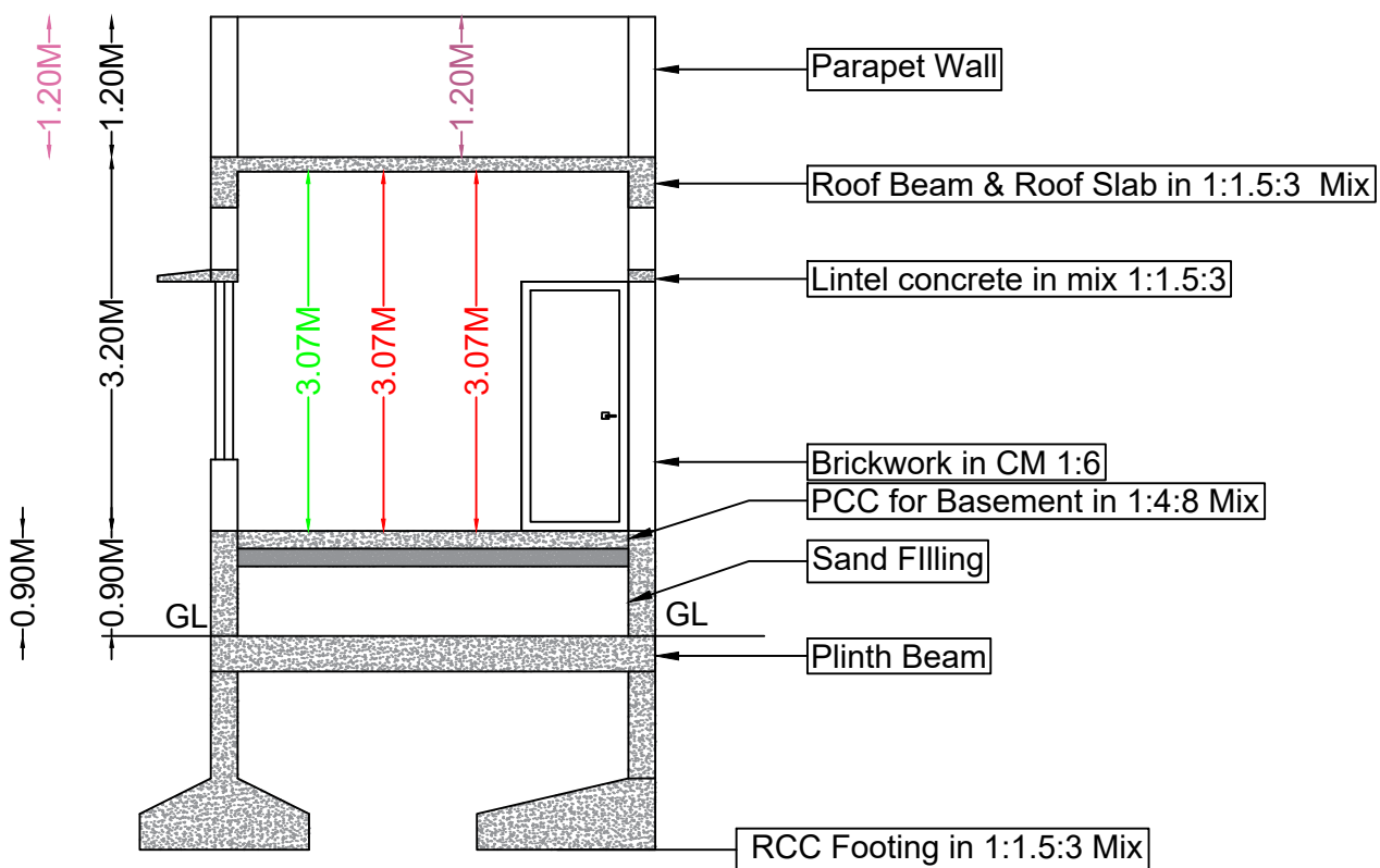
SECTION AB
