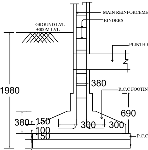
FOUNDATION DETAILS
