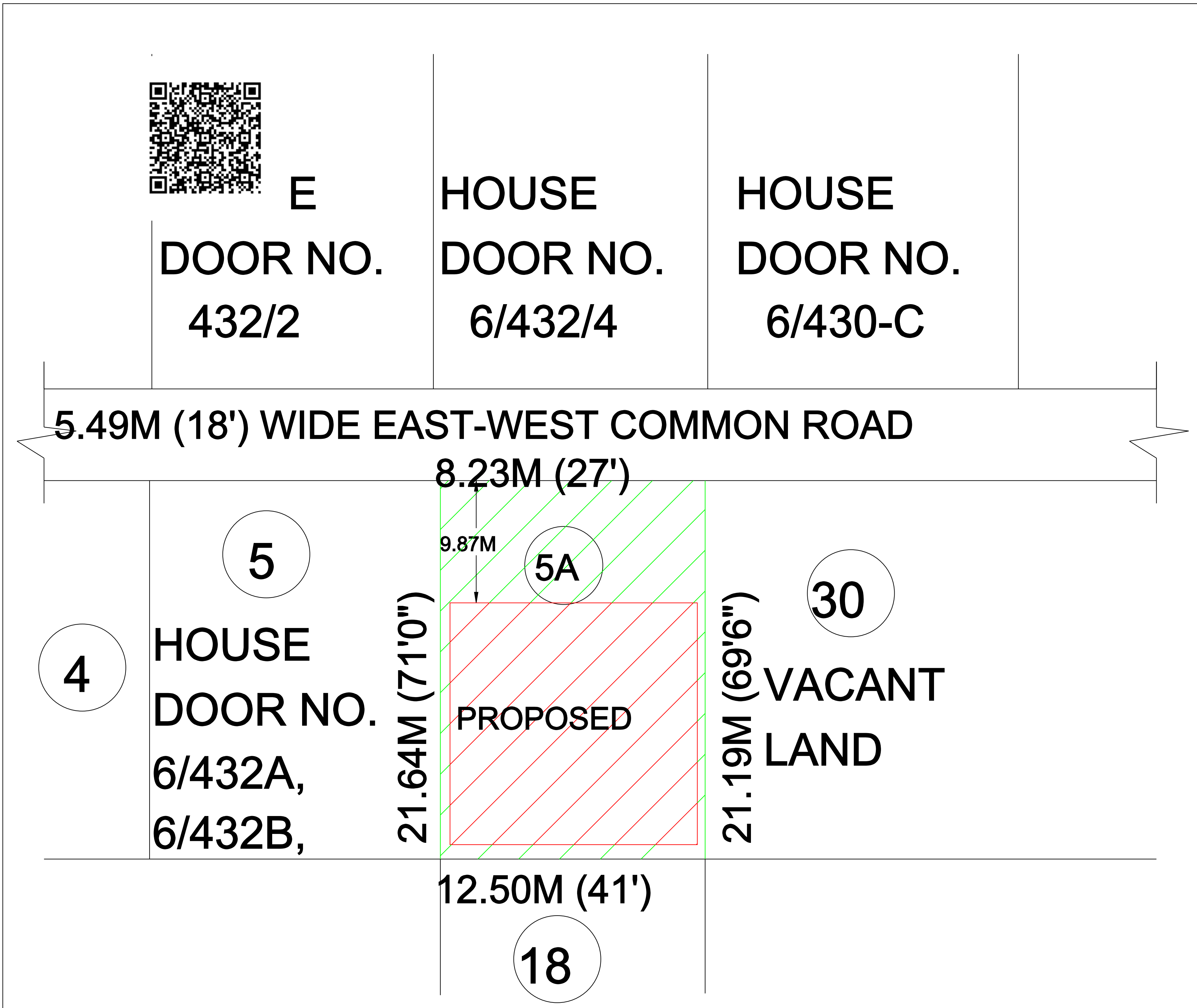
LOCATION PLAN
