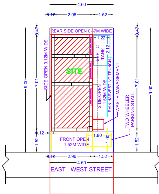
SITE PLAN
