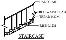
STAIRCASE
