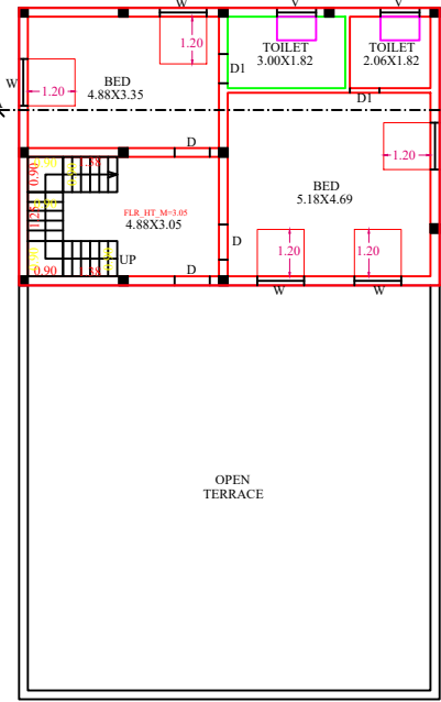
FF PLAN
