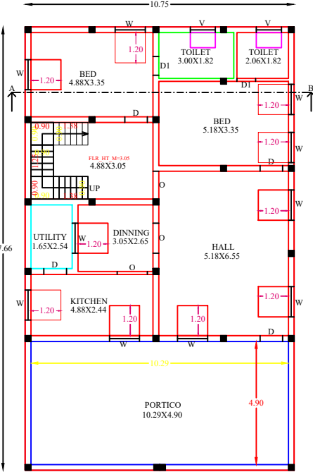
GF PLAN
