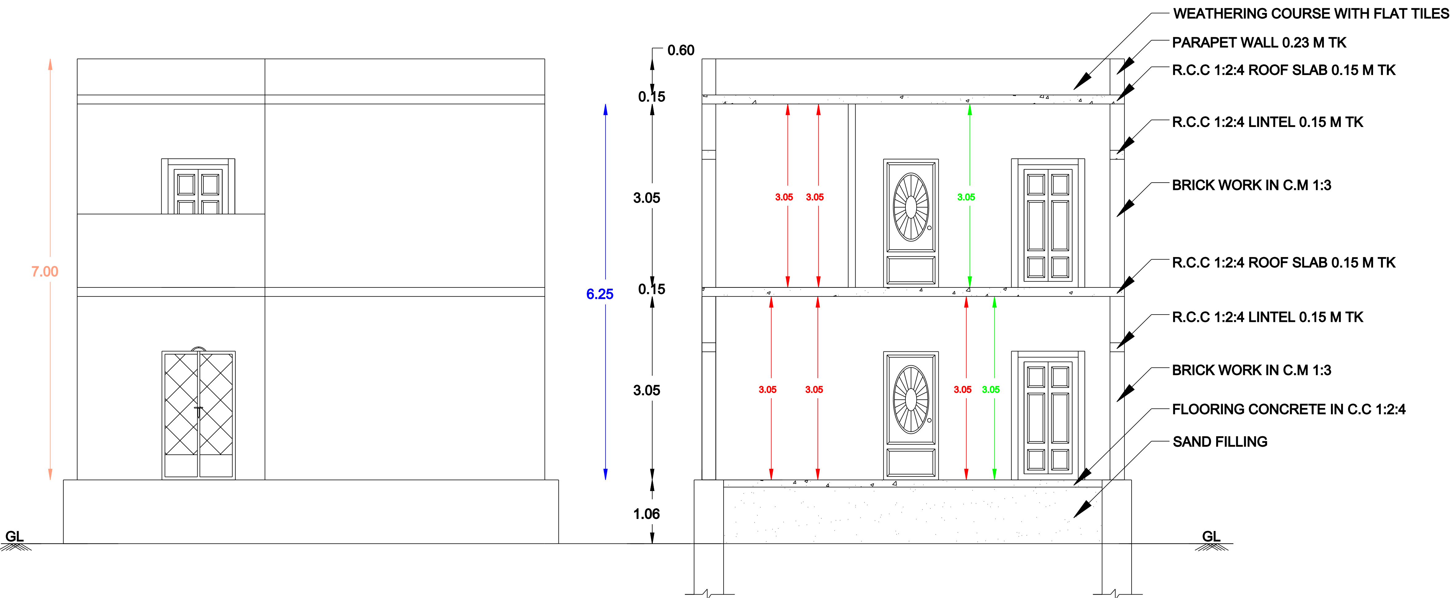
FRONT ELEVATION
