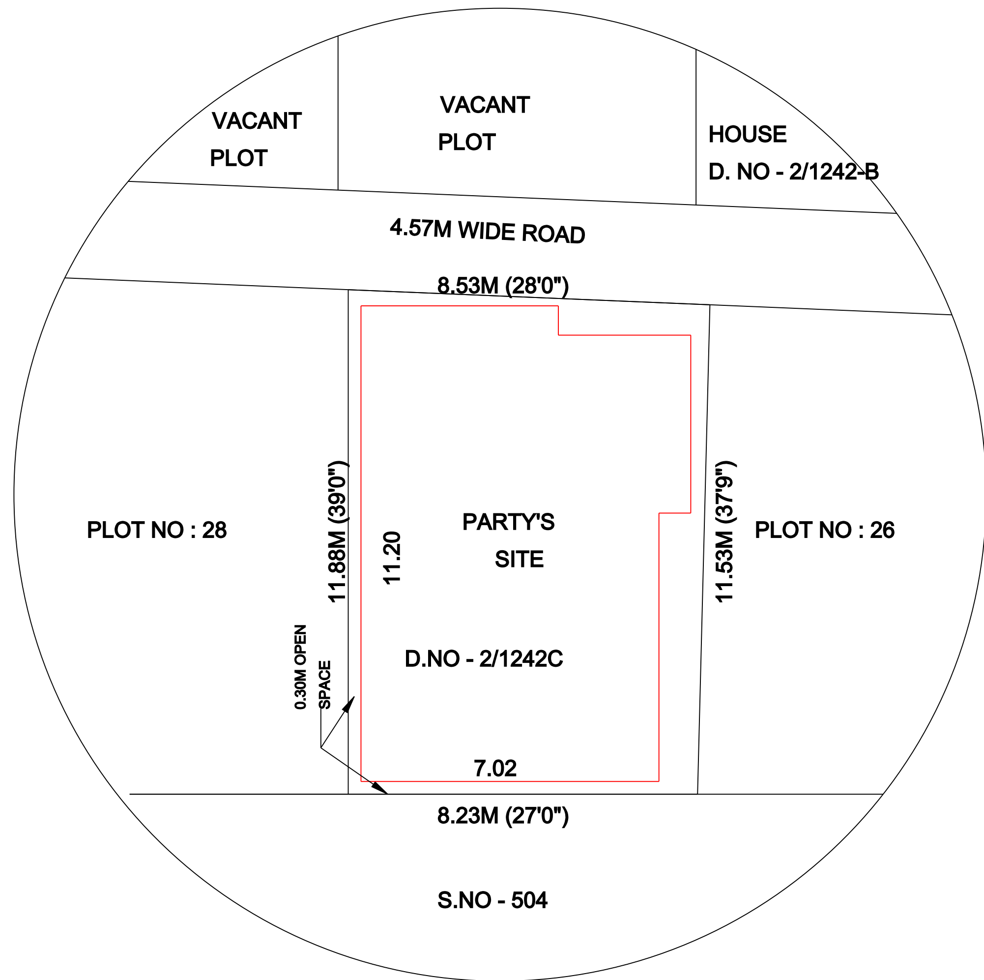
SITE PLAN
