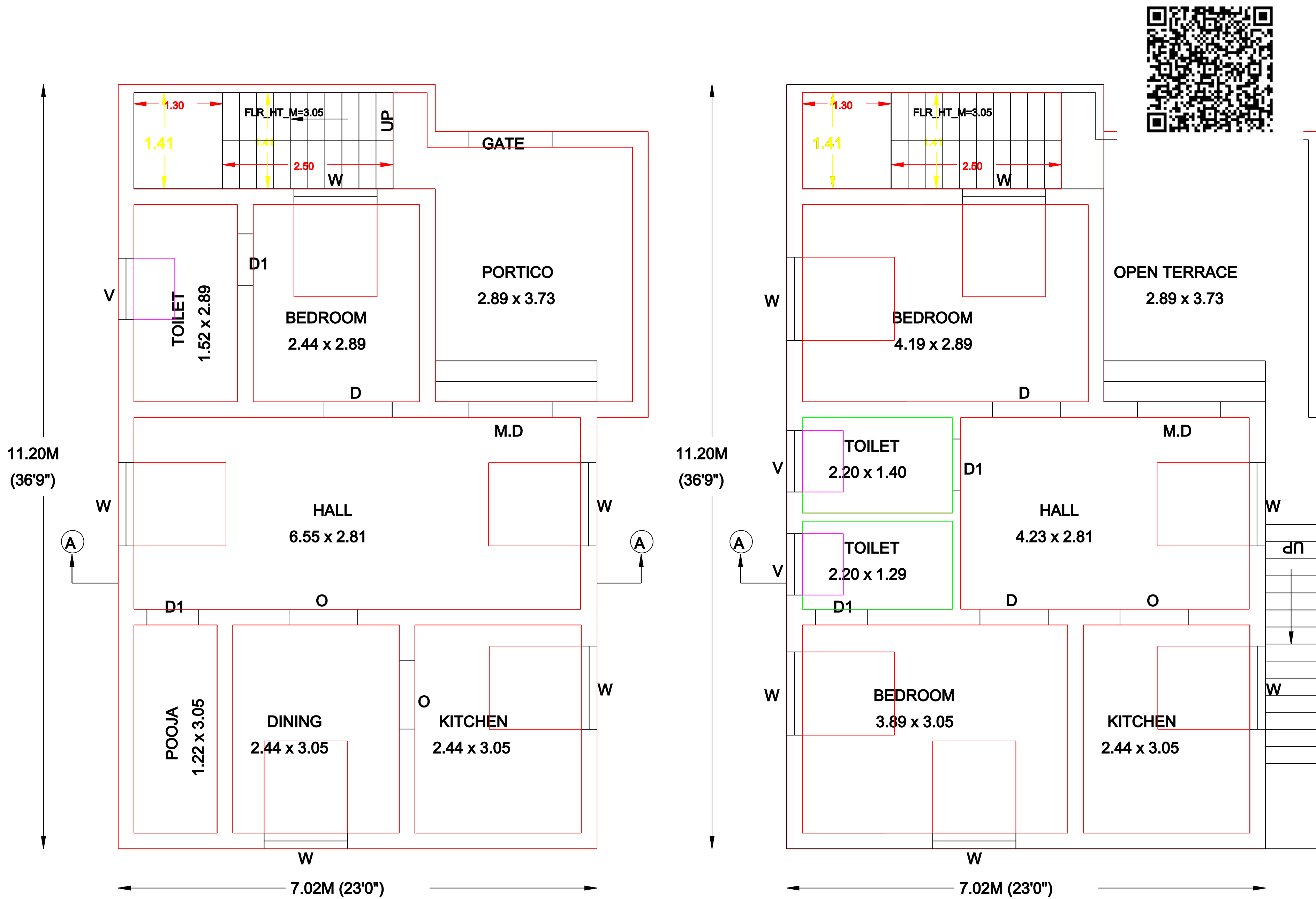
EXISTING GROUND FLOOR PLAN
