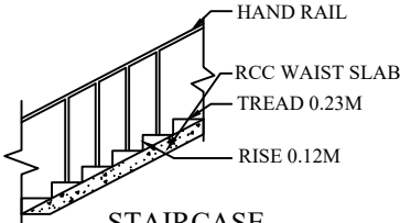
STAIRCASE
