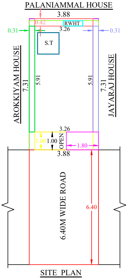
SITE PLAN
