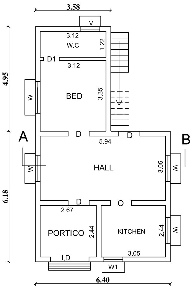
PLAN
