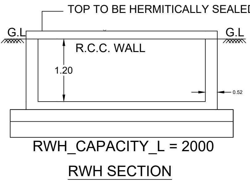
RWH SECTION
